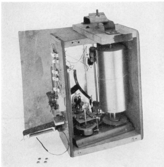
1. Revolving drum to record the lift developed in static tests in the 20-foot tower.
