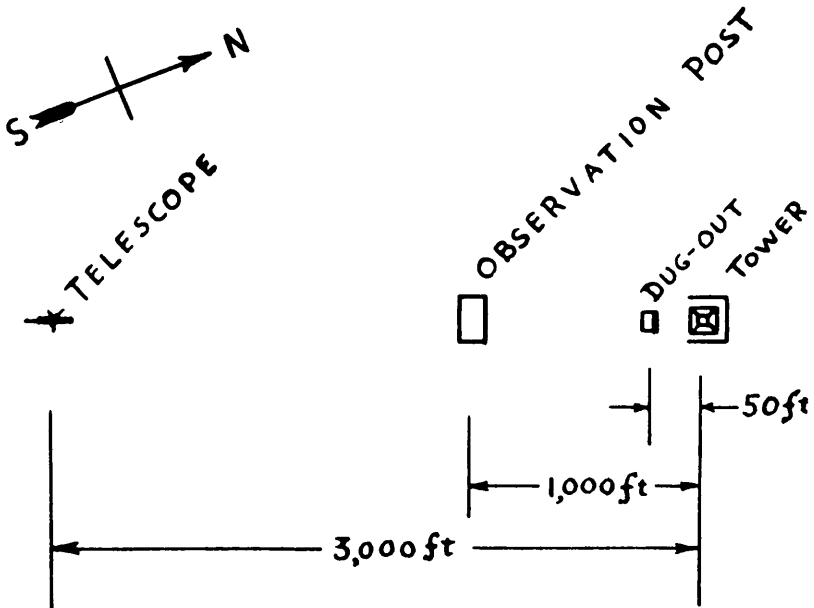
FIG. 1.—Relative positions of launching tower, dugout, shelter, and telescope.
