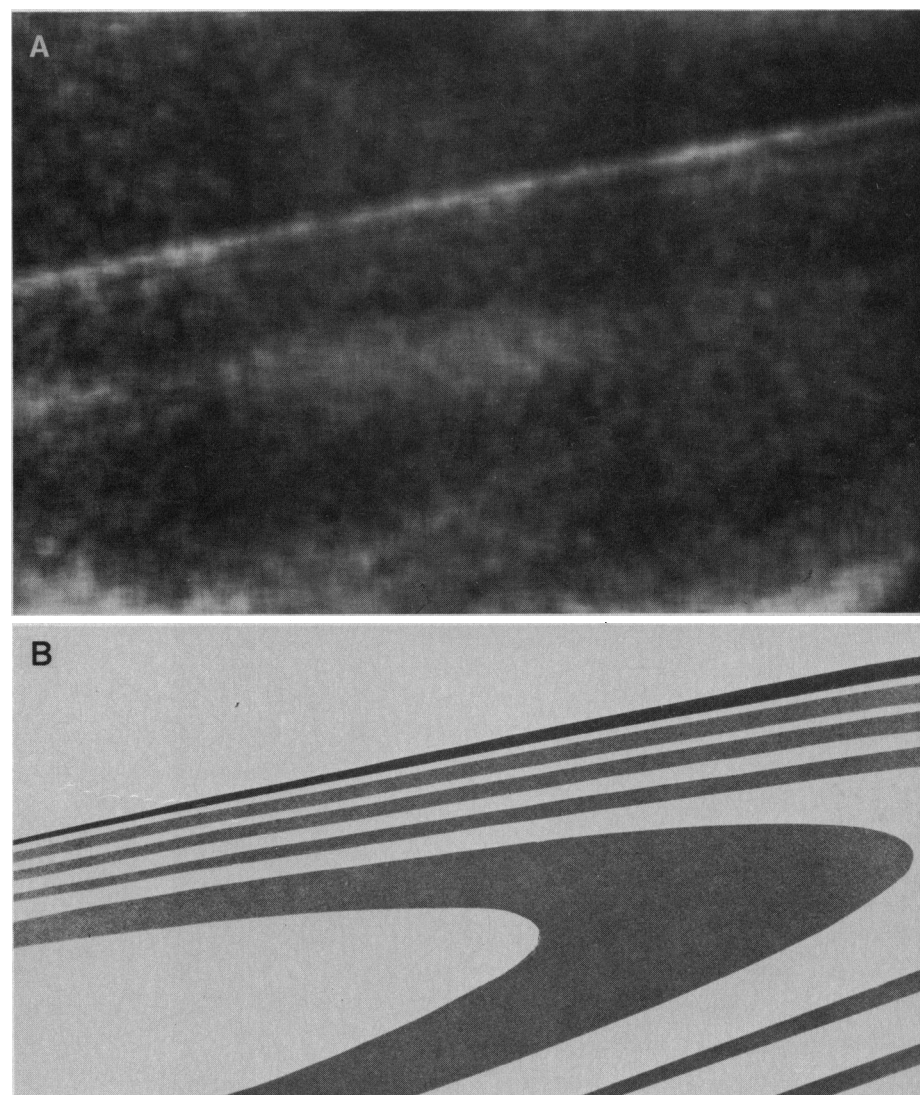
Fig. 11. (A) Enhanced wide-angle image of the region inside the main rings, revealing a broad disk of material. Part of the ring-plane crossing sequence, this image was acquired from a subspaceship latitude of 4^\circ and a phase angle of 90^\circ and with an exposure time of 7.68 seconds. The image contains about 15 pixels of smear predominantly in the direction perpendicular to the ring plane. (B) Viewing and illumination geometry of this image.
