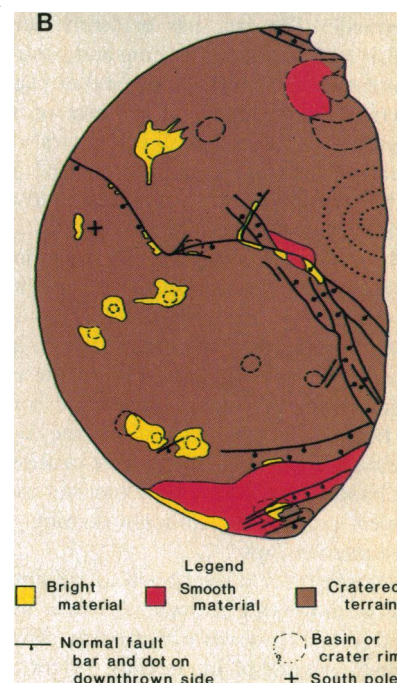
Fig. 23. (A) Voyager 2's highest resolution view of Titania. This image was high-frequency filtered to enhance details. The resolution is about 7 km per line pair, and the phase angle is about 35°. (B) Geologic sketch map of Titania.
