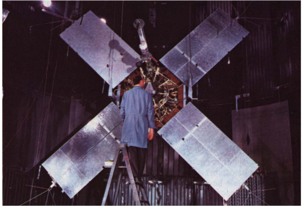
Preparation for test firing of midcourse motor in 25-foot space simulator
