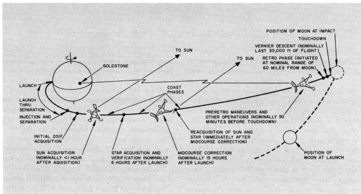
FIGURE 5. — Earth-Moon trajectory and nominal events.
