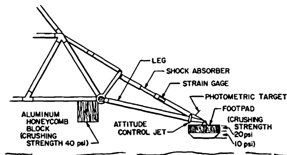
FIGURE 8. — Drawing of landing-leg assembly 2.
