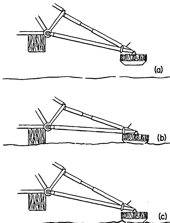
FIGURE 9. — Schematic of the Surveyor landing-leg assembly showing the articulation in a sequence of events during landing. In (a), the assembly is fully extended. During a landing, the shock absorber compresses and the footpad moves up and away from the spaceframe, as shown in (b). In (c), the assembly is shown reextended after landing.
