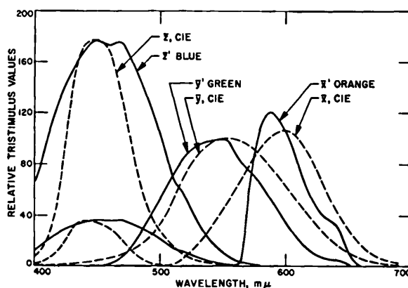
FIGURE 19. — Graph of the overall camera-filter spectral response illustrating the fit to the standard CIE (Commission Internationale l'Eclairage, 1931) color-matching functions. The second maximum in the \bar{x}' curve is obtained from a reduced value of the \bar{z}' function added to the original \bar{x}' camera-filter response. Solid lines are camera-filter response curves; dashed lines are CIE color-matching function.
