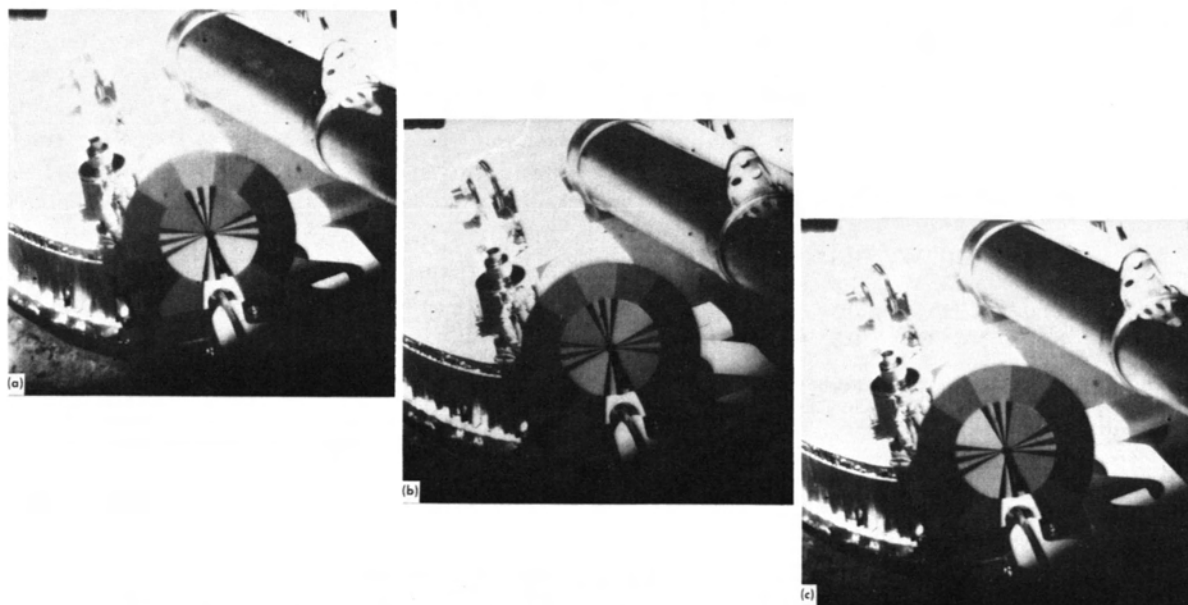
FIGURE 20.— Photometric target on footpad 2 of the Surveyor spacecraft. The target is used for photometric calibration of the television camera during lunar operation. Frame (a) is observed through \bar{x}' filter, (b) is observed through \bar{y}' filter, and (c) is observed through \bar{z}' filter.
