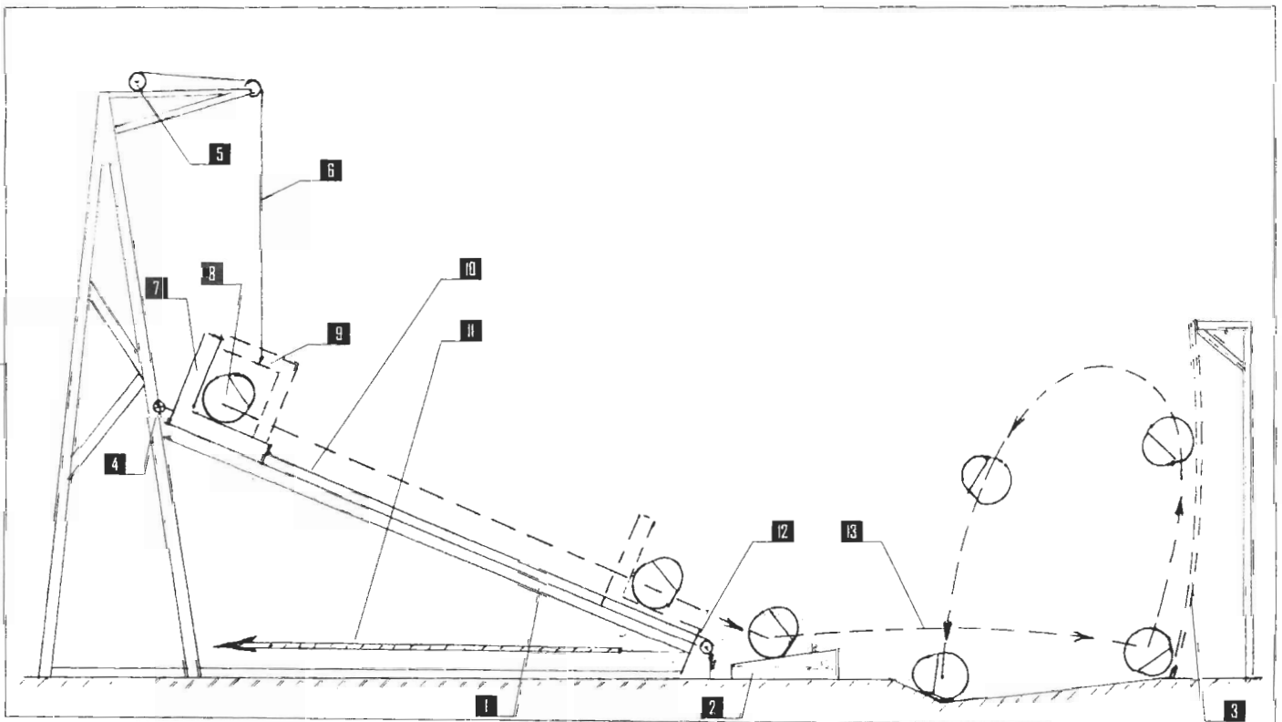
Figure 15. The General Scheme of the Catapult—(1) catapult, (2) platform with the duplicate soil, (3) protective screen, (4) lock, (5) winch, (6) rope, (7) sledge-thermostat, (8) automatic Martian station, (9) top of the thermostat, (10), rope, (11) elastic shock absorber, (12) stopper, and (13) trajectory of the automatic Martian station after it hits the platform ( \alpha —angle of catapult slopes inclination, \beta —angle of the platform inclination)
