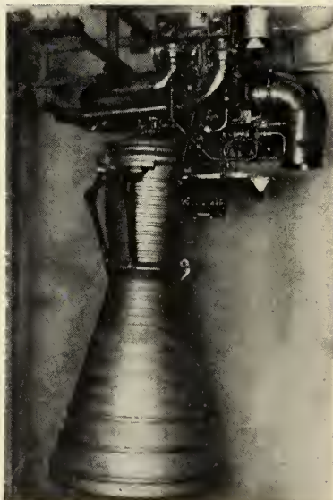
ROLLS-ROYCE rocket engine, similar to those to be tested at Spadeadam, developed for the Blue Streak LRBMs.
