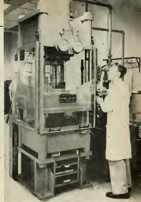
200-TON PRESS is used to press the reduced powders of \text{Al}_2\text{O}_3 and matrix metal.
