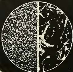
Left: Millipore Filter Right: Dense analytical filter 100 X
