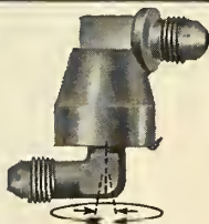
NEW SELF-ALIGNING SWIVEL JOINT— 360° rotation plus 15° side flexibility.
