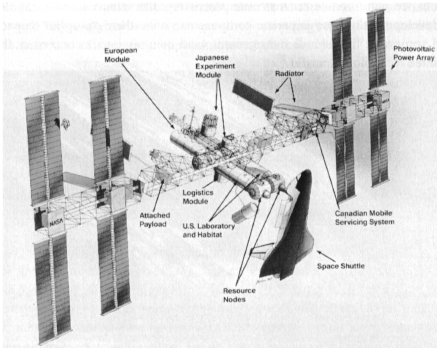
Figure 23-3: This is the baseline configuration of Space Station Freedom , as conceived in 1991. It was published in the booklet, Space Station: A Research Laboratory in Space (NASA PAM-512, n.d.).
