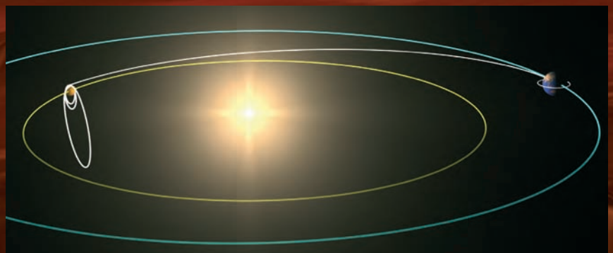
Venus Express's journey to Venus
