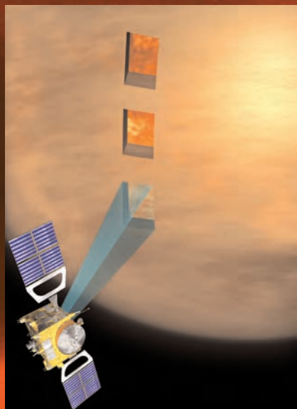
By digging into the atmosphere, Venus Express will provide clues about the whole planet
