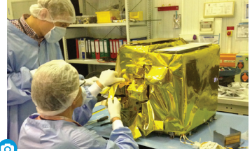
Atmospheric Chemistry Suite (ACS) flight model http://exploration.esa.int/mars/57472
