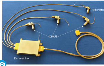
COMARS+ flight hardware http://exploration.esa.int/mars/57379
