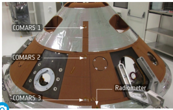
COMARS+ sensors on Schiaparelli http://exploration.esa.int/mars/57377
