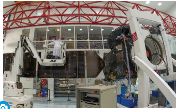
Deployment test of the Trace Gas Orbiter solar arrays http://exploration.esa.int/mars/56917
