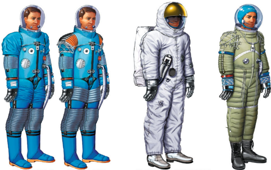
(X) ILC AX5L competition suit (6/65) (a) External view (b) Without covers (Y) HS PLSS and HS/DCC TMG development (6/65–9/65) (Z) HS XT5 (7/65)
