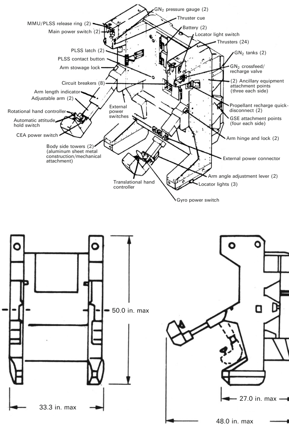
Figure 10.1.14. Features and dimensions of the manned maneuvering unit (MMU) (courtesy NASA).
