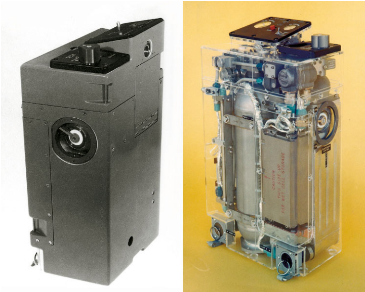
Figure 5.6.3. The AiResearch ELSS (courtesy Honeywell).
