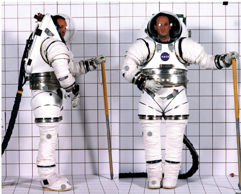
Figure 11.3.9. NASA/ILC hard/soft element hybrid H-suit (courtesy NASA).
