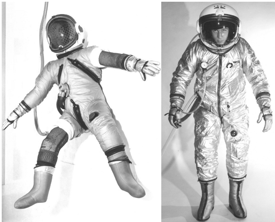
Figure 8.1.2. DCC X-20 “Dyna-Soar” suit configurations (courtesy, left and right, Hamilton Sundstrand and G. L. Harris, respectively).
