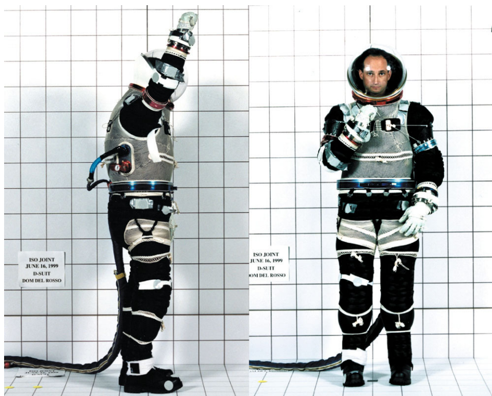
Figure 11.3.13. DCC “D” lunar/Mars soft suit (courtesy NASA).
