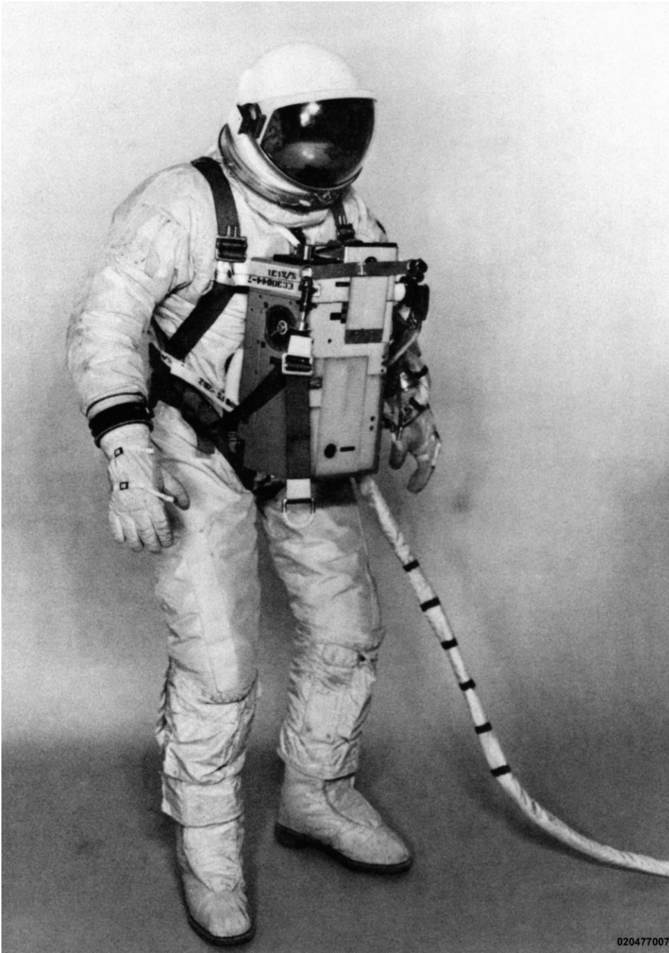
Figure A.5. Gemini V to XII DCC G4C suit and AiResearch ELSS (courtesy NASA).
