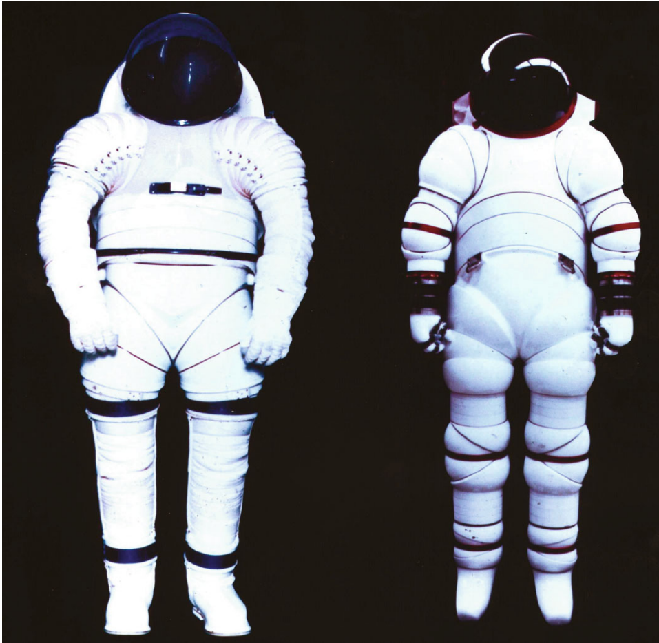
Figure 11.1.15. Testing JSC's Mark III (left) and Ames' AX-5 (right) (courtesy Hamilton Sundstrand).
