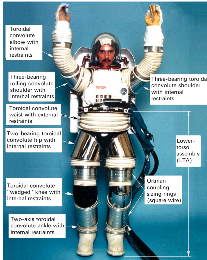
Figure 11.1.2. A typical ZPS test configuration (courtesy Hamilton Sundstrand).
