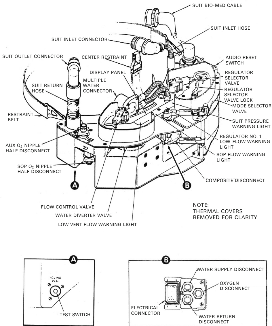
Figure 9.3.3. PCU features (courtesy NASA).
