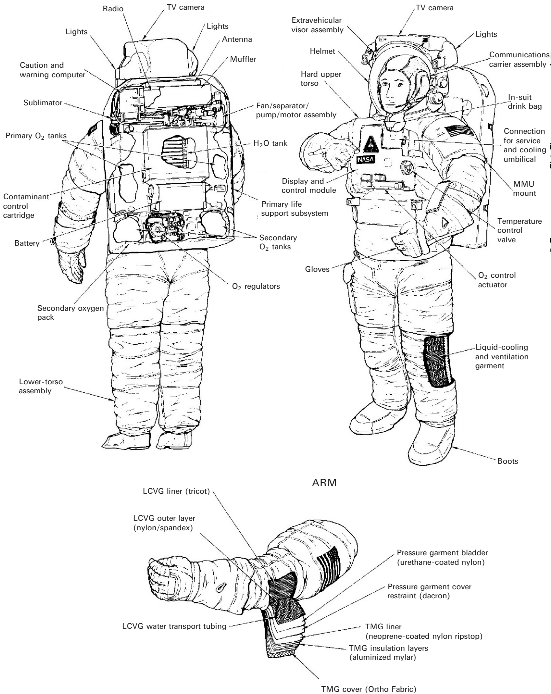
Figure 10.2.2. Shuttle EMU explanation diagram (courtesy Hamilton Sundstrand).
