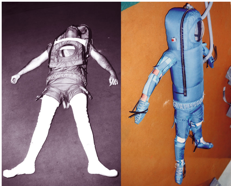
Figure 8.4.7. 1969 human testing of SPCA suit (courtesy Hamilton Sundstrand).
