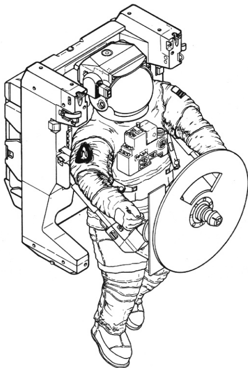
Figure 10.1.15. MMU with satellite attachment devise (courtesy NASA).
