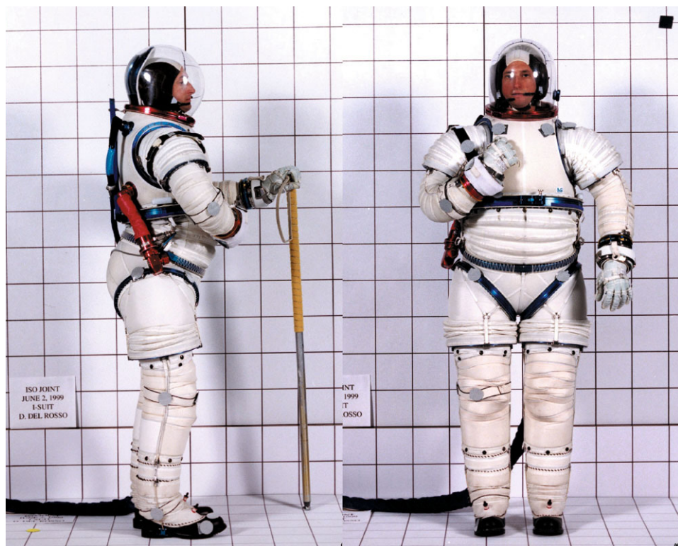
Figure 11.3.11. ILC “I” lunar/Mars soft suit (courtesy NASA).
