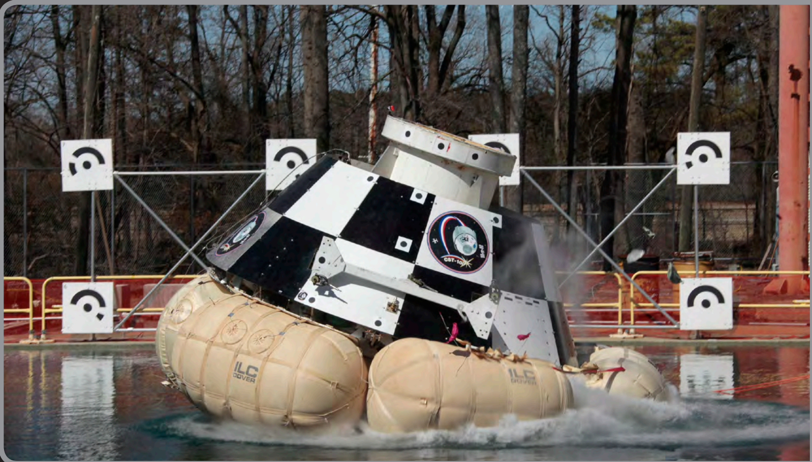
A mockup of Boeing's CST-100 Starliner splashes into a water tank at NASA's Langley Research Center in Virginia during landing system testing. Photo credit: NASA Langley
