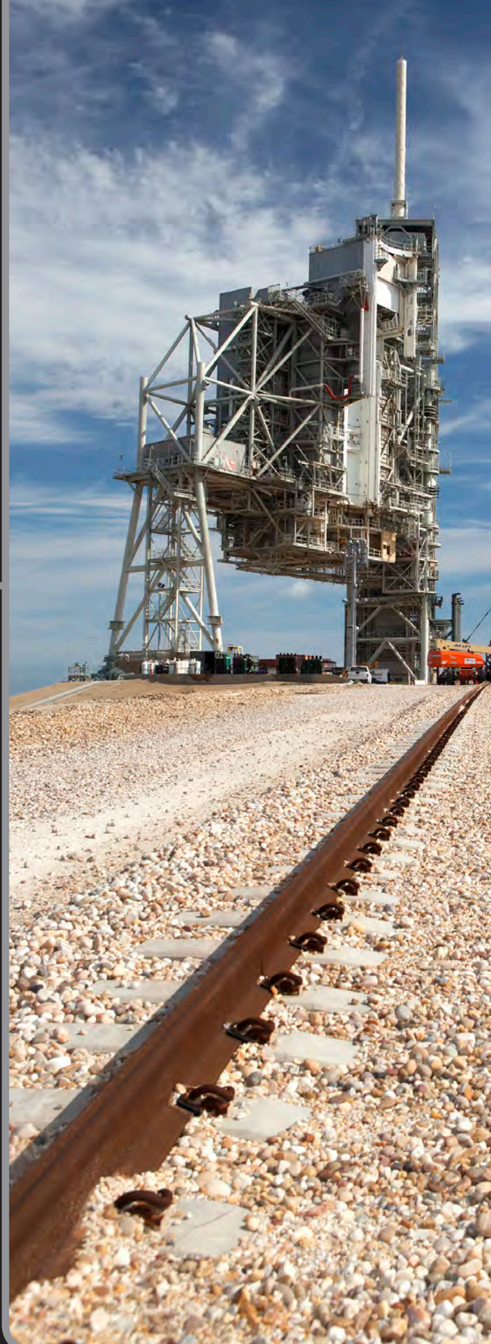
Boeing and United Launch Alliance constructed a Crew Access Tower at Space Launch Complex 41 to give astronauts access to the Starliner spacecraft as it stands atop an Atlas V rocket for liftoff. Photo credit: NASA/Charles Baker
