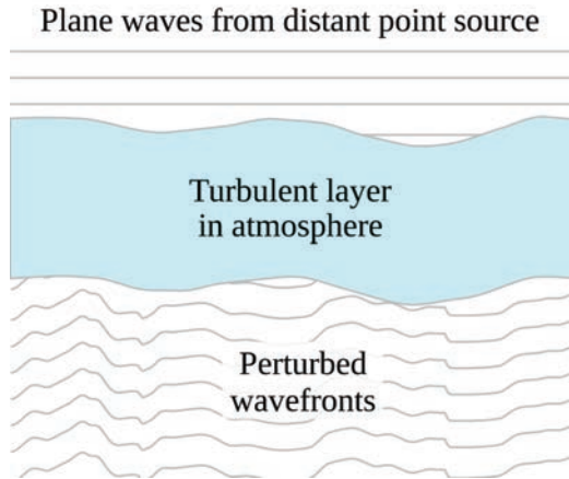
Fig. 2.9: The wavefront perturbed by the turbulent atmosphere of the Earth causes images of distant objects to be distorted
