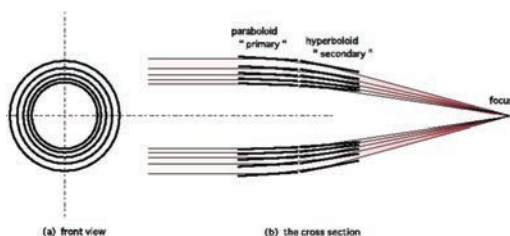
Fig.7.3: Wolter-I geometry
