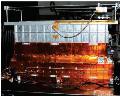
Fig.7.5: View of LAXPC
