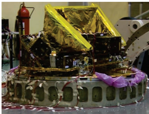
Fig.7.8: View of SSM
