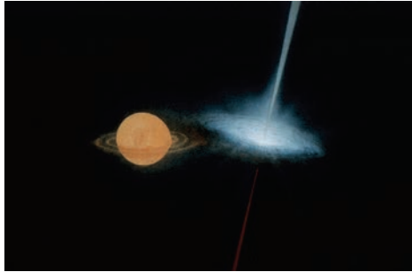
Artist's rendition of a micro-quasar (Source: Wikipedia)
