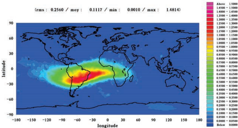
Fig. 2.14: The South Atlantic Anomaly
