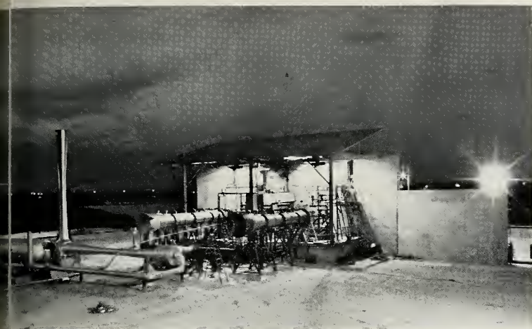
WILIGHT VIEW of Pratt & Whitney's double test stand for liquid hydrogen rocket engines showing the big tubes through which the engines fire.
