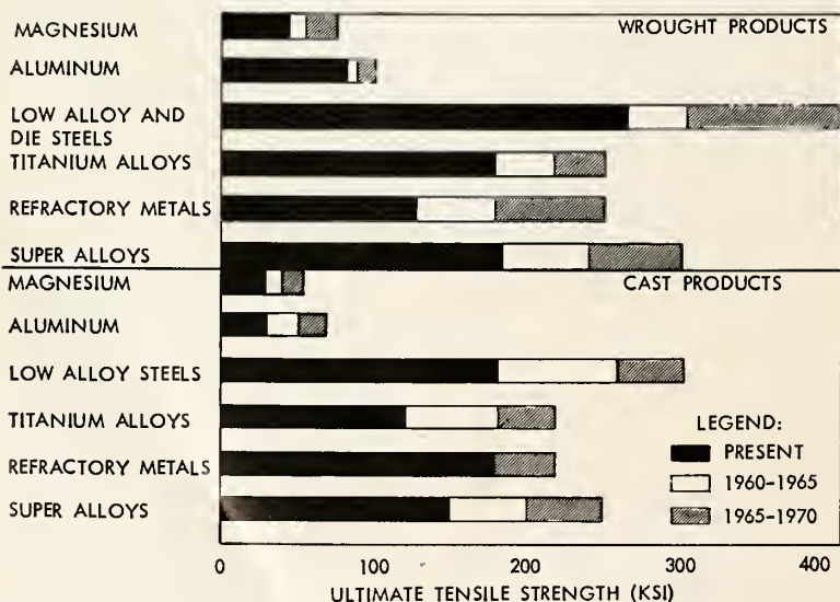
ANTICIPATED increase in mechanical properties of wrought and cast alloys.
