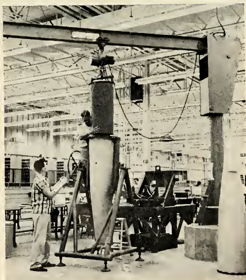
A CANISTER is installed in the nose section of a Lacrosse missile, in production at Martin-Orlando. Lacrosse equipment was delivered recently to Army at Ft. Sill, Okla.
