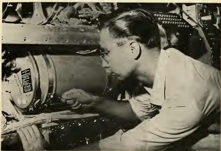
ELECTRIC Silvercel battery by Yardney is being installed in an Air Force ICBM, to supply main power during flight. It discharges 300 amps at 26 volts for 10 minutes.
