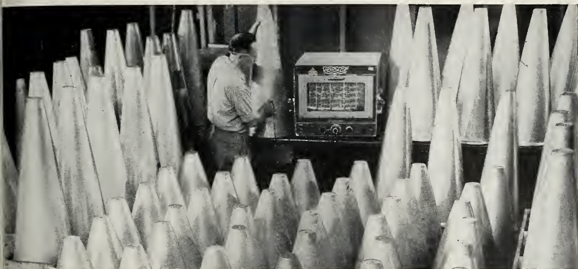
EXAMPLE of inter-industry cooperation in Connecticut is use of ultrasonic resonance gage developed by Branson Instruments, Inc., of Stamford, to test wall thickness of Nike-Hercules nose cones built by Avco's Lycoming Division, Stratford.
