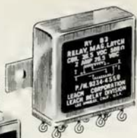
TYPE 9234-4550 2PDT, 2AMP, MAGNETIC LATCH RELAY
