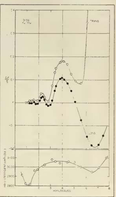
UNUSUALLY high magnetoresistance \Delta P/P_0 and the Hall coefficient determined by NBS for n-type indium-antimonide at 1.7°K are shown.
