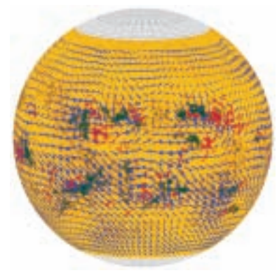
'Solar Subsurface Weather' map, showing magnetic field (black/red) and average 'wind' flow (blue arrows) under the solar surface
