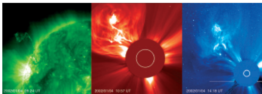
This fiery coronal mass ejection shows stunning details in the ejected material, revealed by SOHO's LASCO coronagraph. The direct sunlight is blocked (red disc), exposing the surrounding faint corona. The white circle represents the approximate size of the Sun
