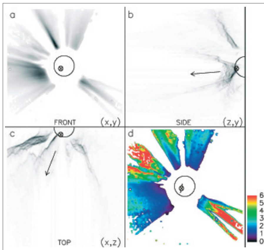
A coronal mass ejection heading almost directly towards Earth, observed by LASCO C2. The size of the Sun is indicated by a circle, and the x-marked circle on the Sun shows the origin of the CME. Panel (a) shows the total intensity (darker means more intense) as imaged directly by LASCO. Panel (d) is a topographic map of the material shown in panel (a). The distance from the plane of the Sun to the material is colour-coded; the scale in units of solar radii is shown on the side. Panels (b) and (c) show the intensity as it would appear to an observer positioned to the side of the Sun or directly above it, respectively
