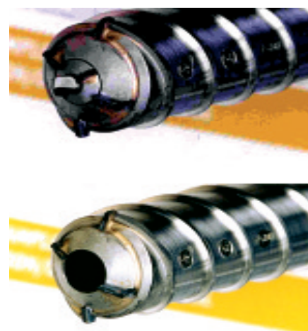
The Pasteur payload's drill-bit design concept. The drill's full 2 m extension is achieved by assembling four sections (one drill tool rod, with an internal shutter and sample-collection capability, plus three extension rods). The drill will also be equipped with an IR spectrometer for mineralogy studies inside the borehole. (Galileo Avionica)
