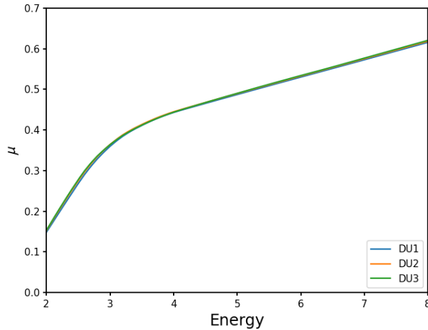
Figure 14: Modulation factor as function of energy for the IXPE DUs estimated at time of IXPE launch. Values are derived from ground calibration data after correcting for spurious modulation and applying weighting.
