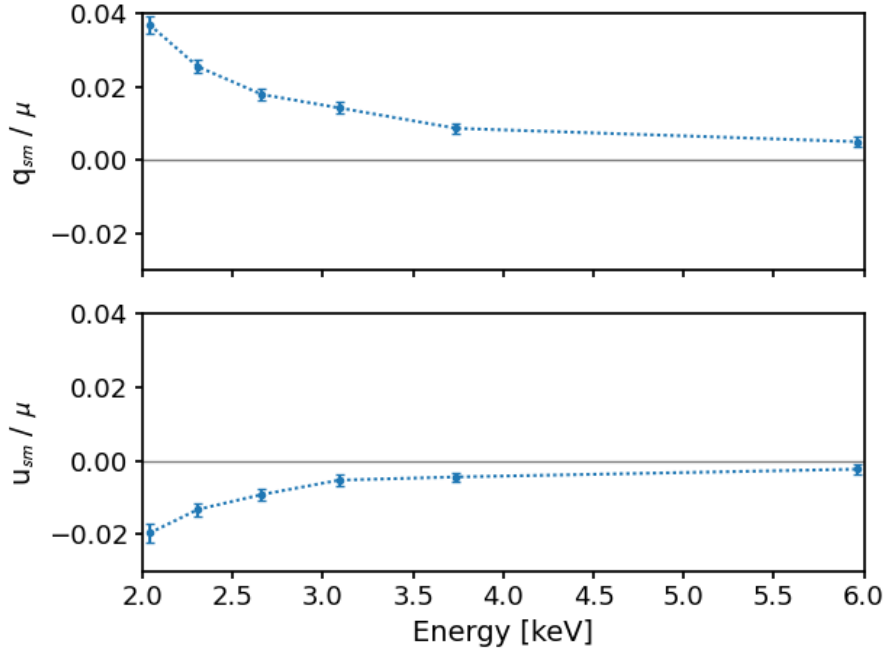
Figure 25: Stokes parameters as a function of energy of the detector-averaged spurious modulation accounting for the 120°clocking of the detectors. The effect is removed during the on-ground data processing.
