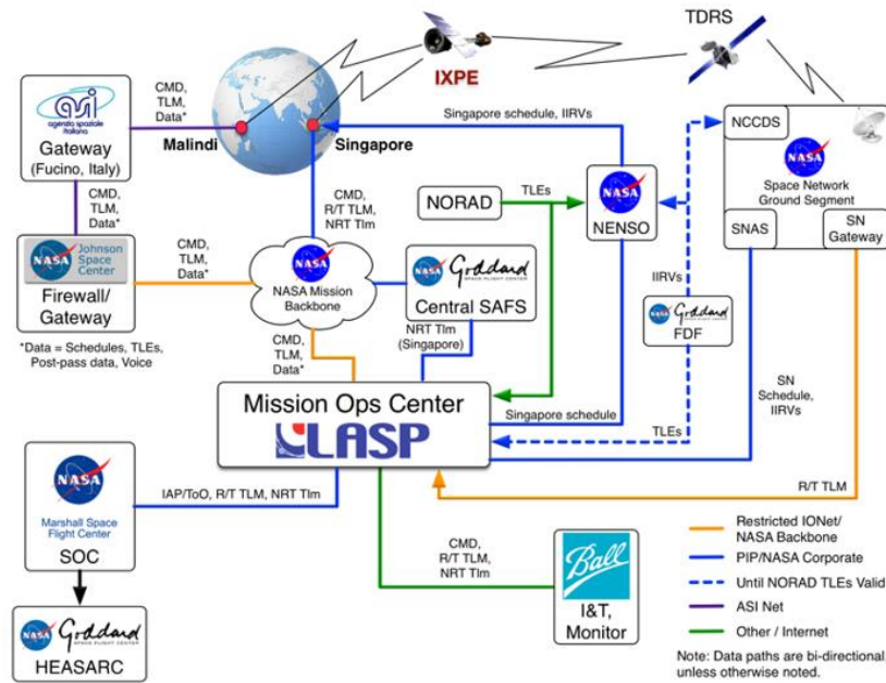
Figure 5: The IXPE ground system. The TDRS is only baselined for use during launch and early operations phases of the mission.
