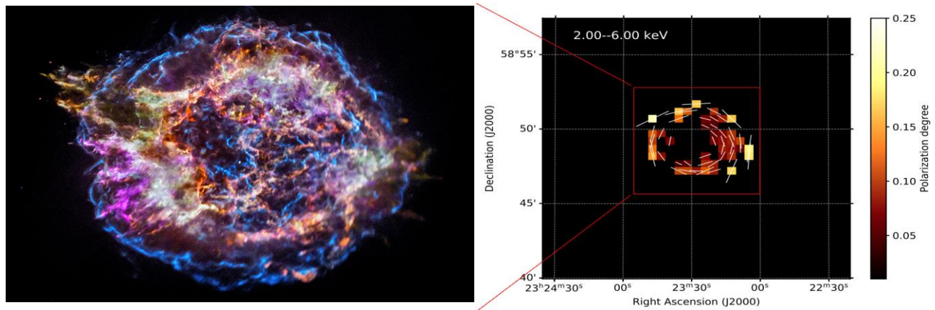
Figure 18: Left: a Chandra X-ray Observatory CCD image of Cas A. Right: IXPE pixels delivering >3\sigma 2-6keV polarization measurements assuming 20% tangential polarization of the non-thermal flux and a 1Ms exposure
