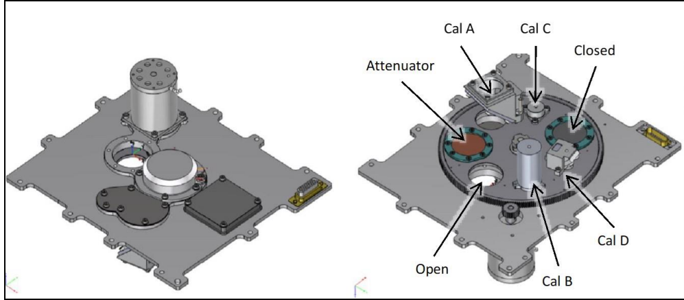
Figure 17: Filter and calibration wheel assembly (left: top view; right: bottom view)
