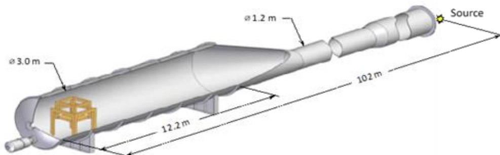
Figure 7: The MSFC Stray-Light Test Facility (SLTF)
