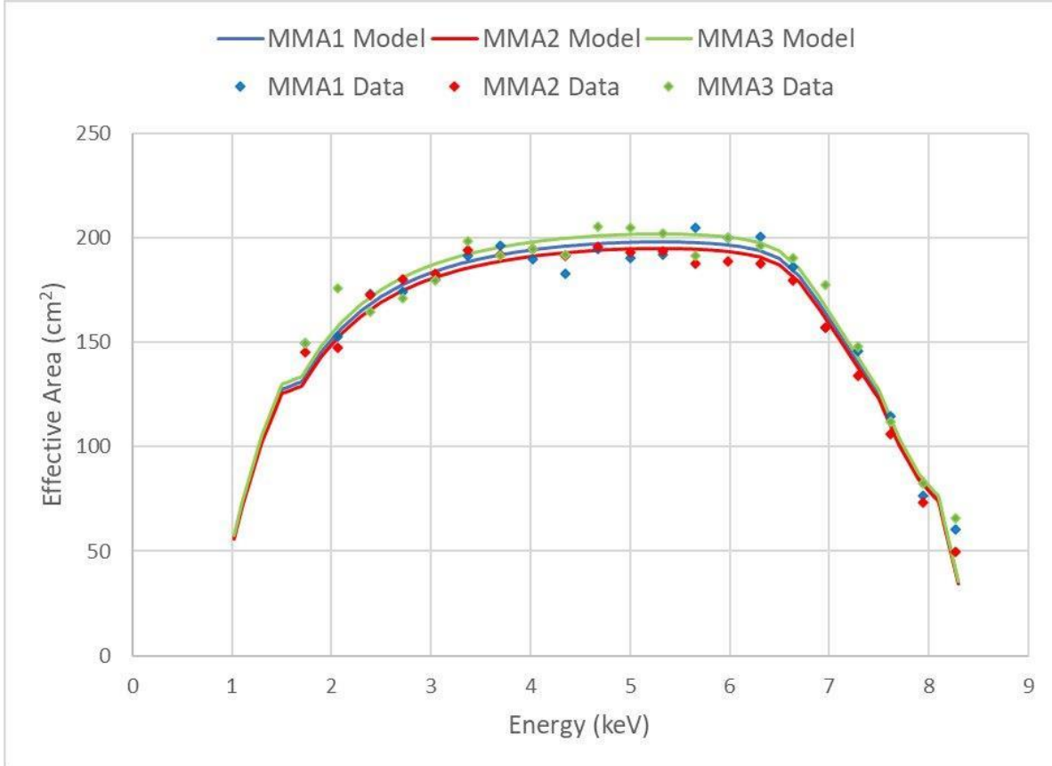
Figure 8: Effective area (measured and best-fit model) for a point source at infinity as a function of energy for the three flight MMAs.
