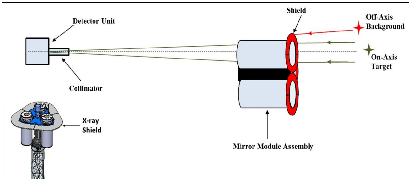
Figure 4: The combination of the forward X-ray shields and the collimator mounted to each detector prevents X rays, other than those passed through the mirror assemblies, from entering the detectors.
