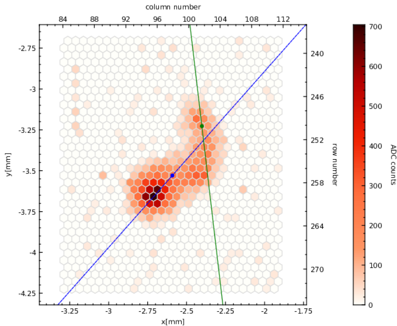
Figure 11: Example of the image of a photoelectron induced track from a 5.9 keV photon. 10 The color scale represents the charge content of each pixel after subtracting a noise floor. The blue line and point represent the principal axis and the barycenter of the track, while the green line and point represent the best estimate of the photoelectron direction and photon absorption point using the moment analysis.
