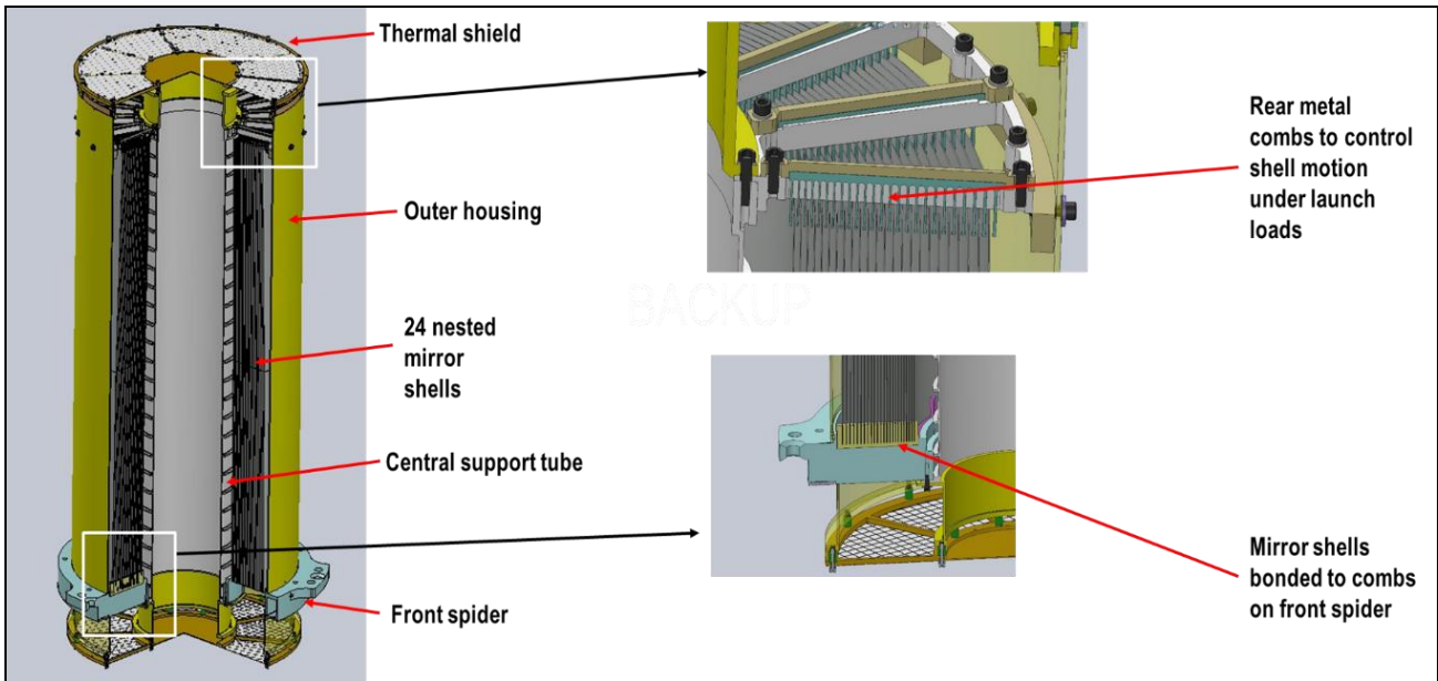
Figure 6: Mechanical design of the Mirror Module Assembly
