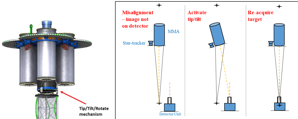
Figure 16: Left image shows the Tip/Tilt/Rotate mechanism; Right image shows the on-orbit alignment process
