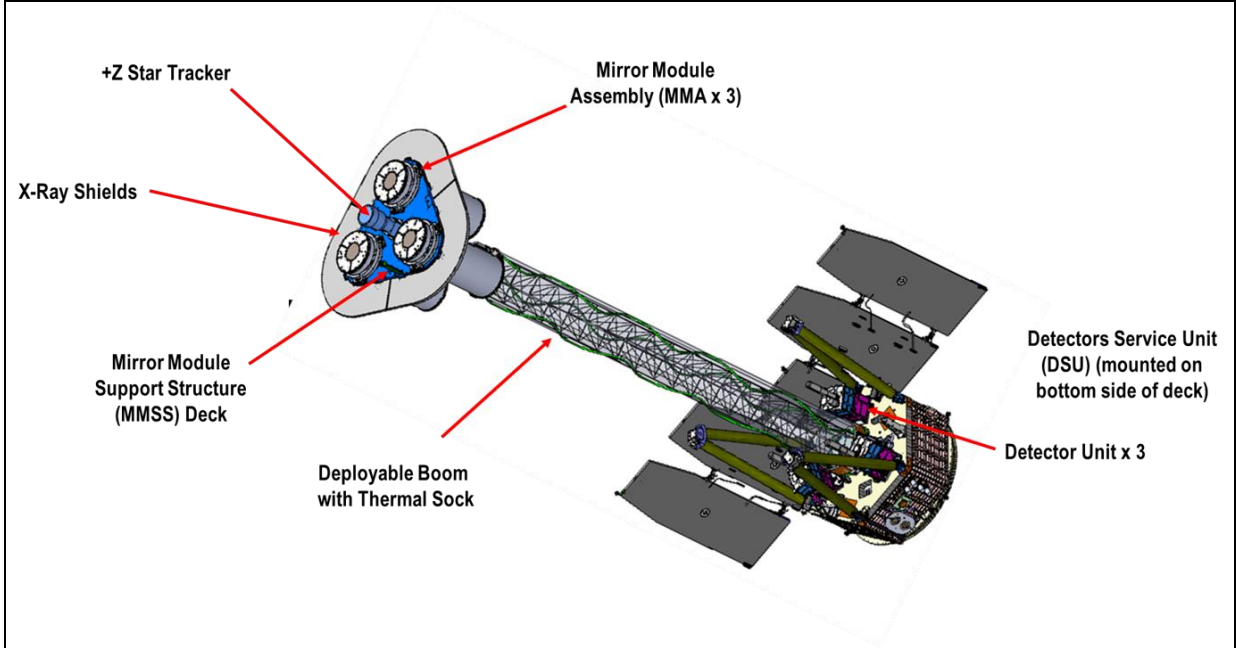
Figure 1: The IXPE Observatory highlighting the key scientific payload elements. A second star tracker (not visible) is on the back of pointing along the -Z axis. The DSU is a computer that provides the interface between the detector electronics and the S/C computer.
