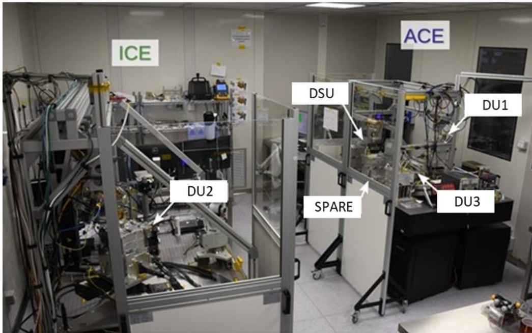
Figure 12: The ICE and ACE calibration stations in Italy during calibration of DU2 flight model on the ICE and the Instrument testing with DSU-EM (Engineering Model) and DU1,3 (flight models) and the spare unit on the ACE.
