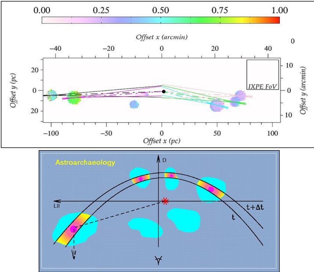
Figure 19: Galactic center schematic (upper), showing a time-delayed scattering signal from the clouds (lower).
