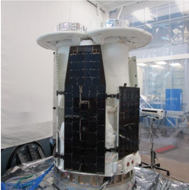
Figure 2: Photograph of the IXPE Observatory in the stowed position on a vibration table during Observatory environmental testing. Photo courtesy of Ball Aerospace.
