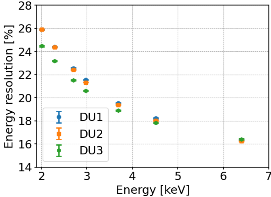
Figure 13: Energy resolution as a function of energy for the flight DUs.
