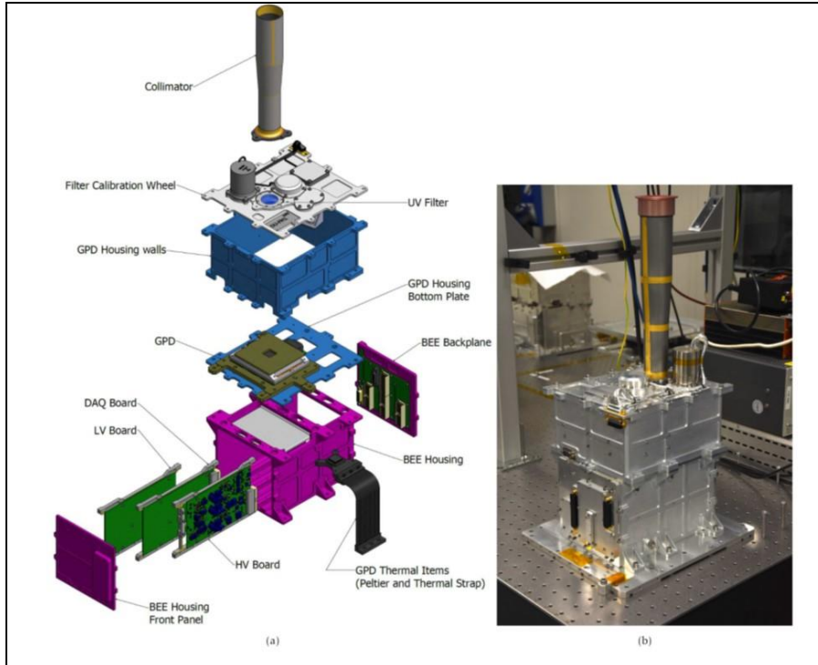
Figure 10: Expanded view of a Detector Unit (DU, left); photograph of a completed flight unit (right).
