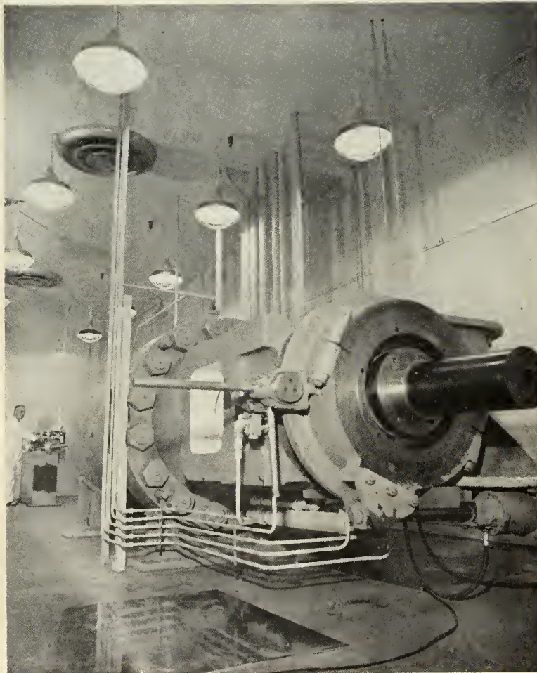
OPERATOR CONTROLS extrusion of ammonium nitrate grain.
