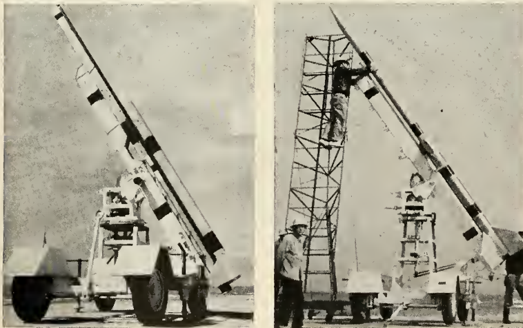
PHOTOGRAPHS AND DATA on the latest Japanese sounding rockets indicate a remarkable advancement in the state of the art. Both of the rockets shown were developed by Professor Hideo Itokawa, Institute of Industrial Science, University of Tokyo. Itokawa is head of Japanese IGY sounding rocket program. K-150 rocket (left). Single-stage, solid propellant sounding vehicle fired April 8, 1958. Diameter—150mm. (5 \frac{1}{2} in.); length—3.3m (10 \frac{3}{4} ft); weight—70kg (154 lbs). Kappa Type V two-stage rocket (right) fired April 29, 1958. First stage diameter—220mm (8 \frac{5}{8} in.). Second stage—K-150 rocket. Maximum velocity—about 1,000 m/sec (3300 ft/sec).
