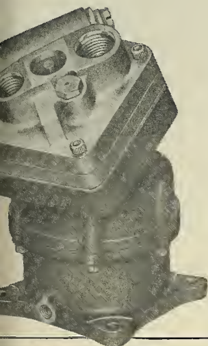
Model Series . . . . . PV062 Theoretical Dspl. .950 cu in./rev *
