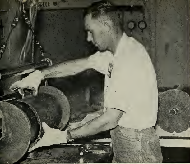
Operator applies combination of sponge pad and buring restrictor to the grain, clamps on metal corset to hold in place during 24-hour curing process. Automatic lathes have been used to bevel grain ends and trim to finished size. Mandrel with wheels is inserted in center core of grain to facilitate movement through curing oven.
