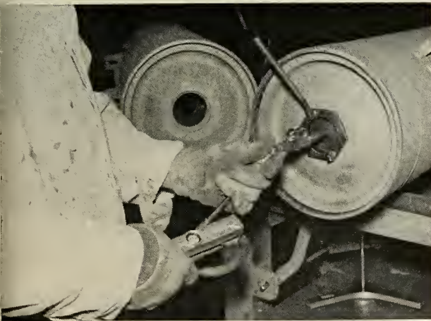
Nozzles are added and units are air tested under 10 pounds of pressure as final manufacturing step. Special shipping plug is installed in the igniter opening while the units are being transported to the field. Company name and identification markings are stenciled on case before it is loaded into shipping case.
