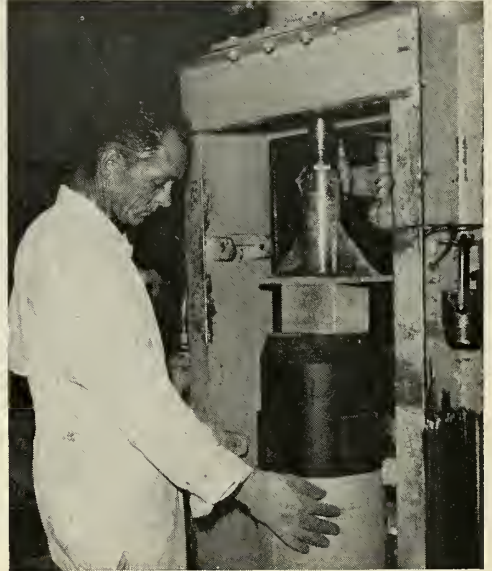
JATO grain and metal case meet for first time at loading station. Here, close-fitting grain is forced into case under 3,500 pounds pressure. Machined steel head is positioned and locked with metal strip key. A rubber O-ring between head and case provides the necessary pressure seal.
