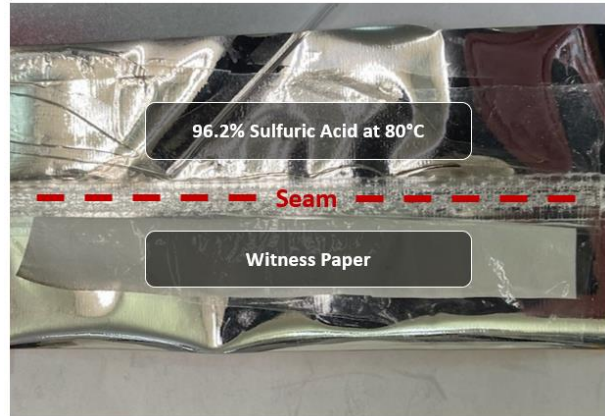
Figure 3: Material coupon test of exterior balloon seam, where a witness paper is protected from acid of same aerosol attributes as present at 52km altitude on Venus.
