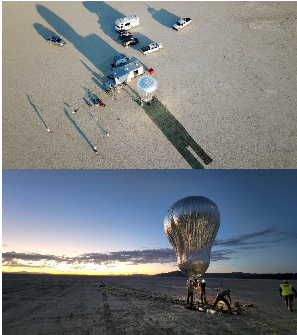
Figure 2: Launch photographs of prototype Venus aerobot during July 2022 test flight campaign. Top: aerial view of first flight in direct sunlight. Bottom: second flight in sunrise radiative flux conditions.
