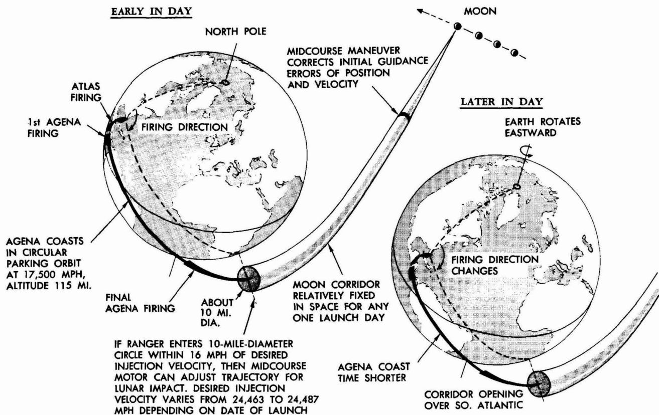
Figure 5. Typical Ranger launch to Moon
