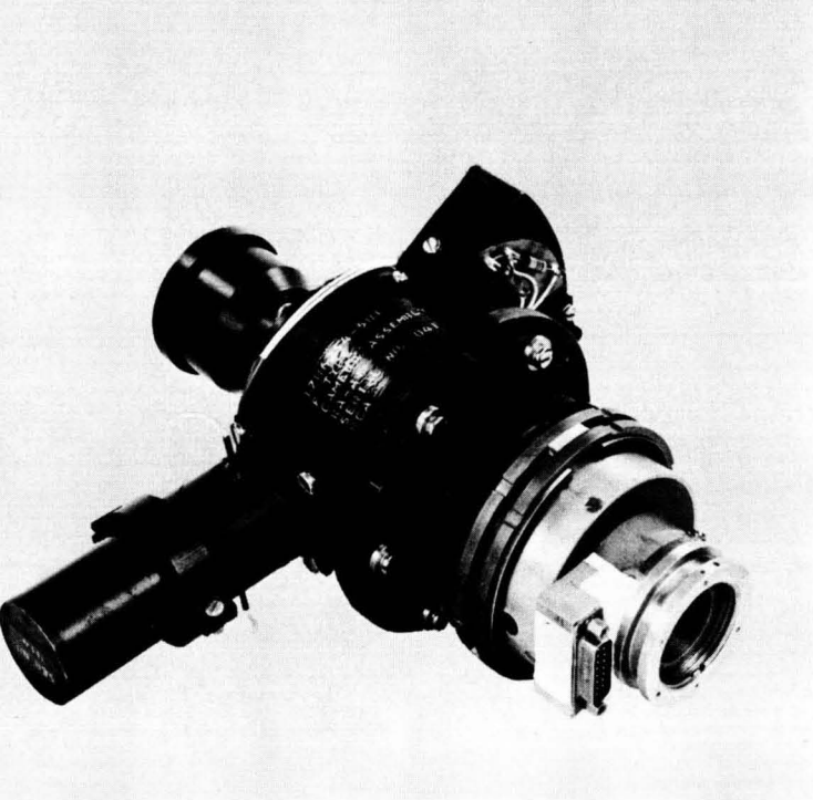
Figure 16. Wide-angle camera of TV system
