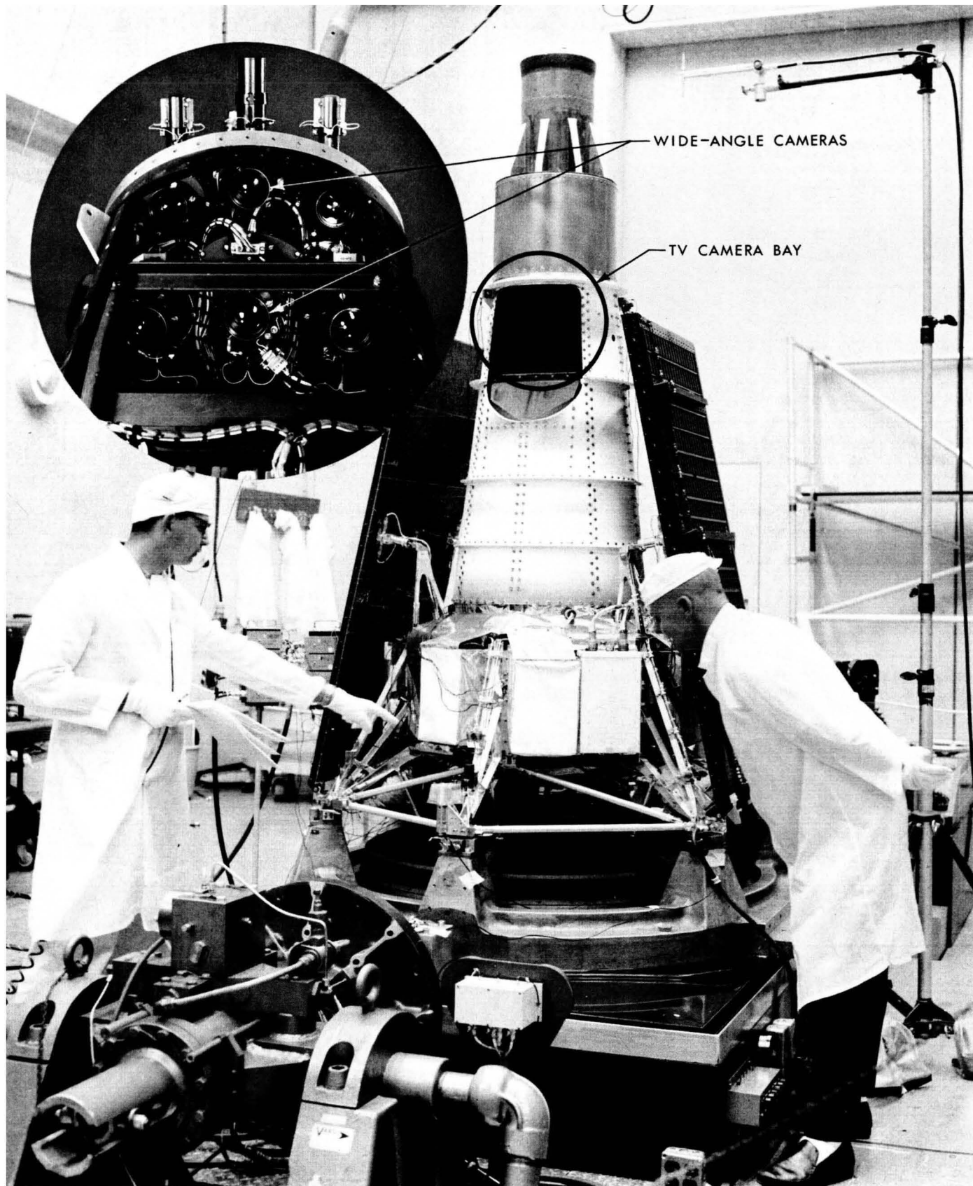
Figure 15. Ranger TV subsystem
