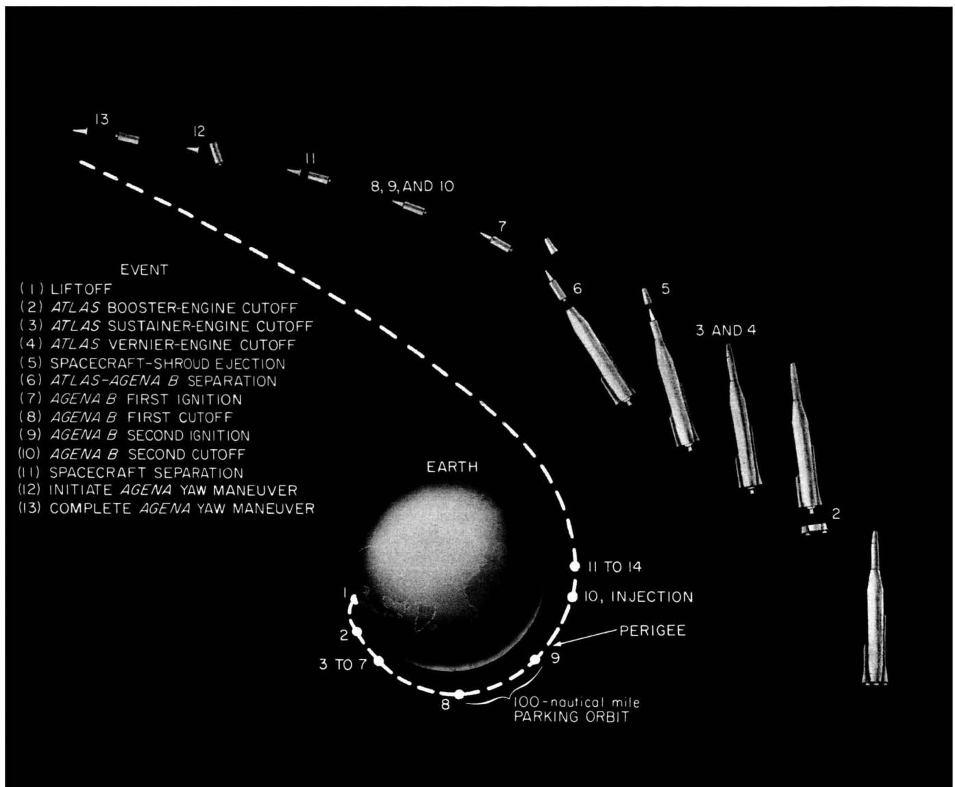
Figure 23. Ranger launch-to-injection events
