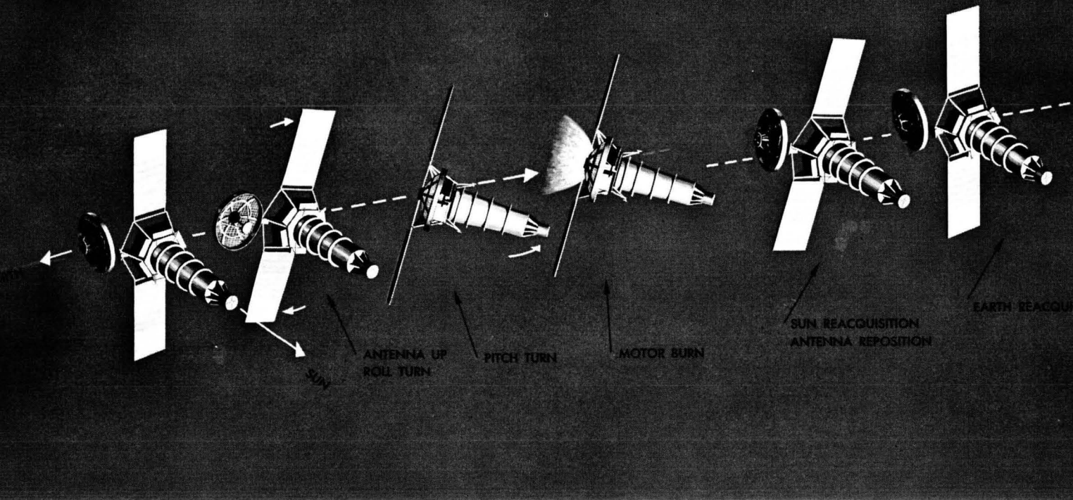
Figure 26. Ranger midcourse maneuver sequence
