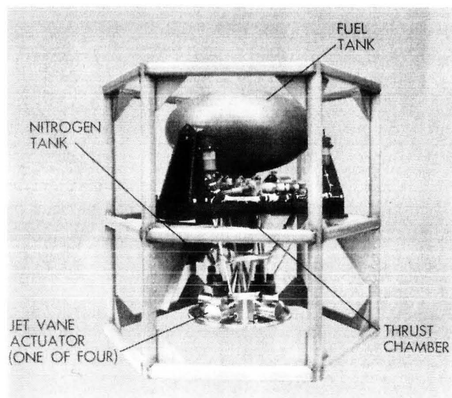
Figure 12. Midcourse rocket motor
