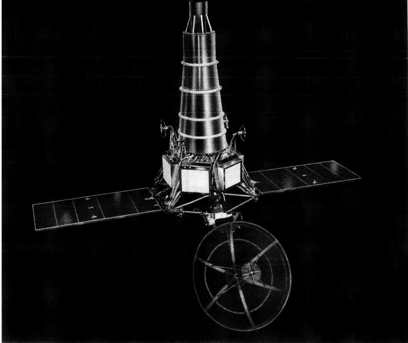
Figure 11. High-gain directional antenna
