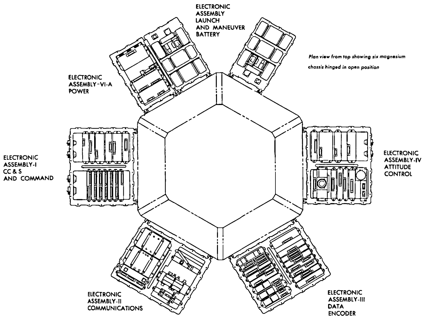
Figure 10. Subsystem cases on spacecraft—hexagonal structure
