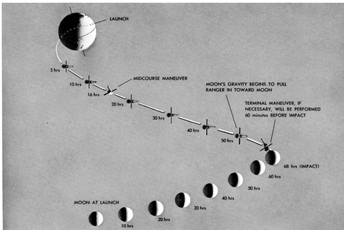
Ranger nominal trajectory to Moon
