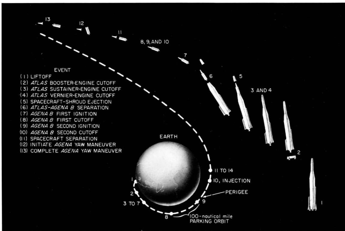
Ranger launch-to-injection events
