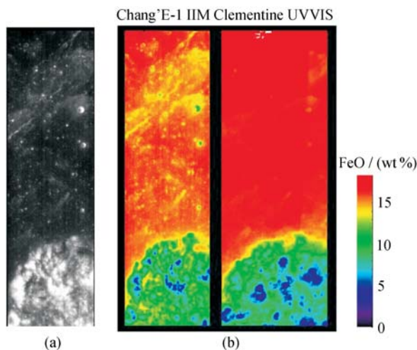
Figure 7 FeO abundance of the lunar surface in the Mare Crisium. (a) Image data was sampled at 757 nm of the 2185 orbit of Chang'E-1 IIM; (b) Iron abundance of the lunar surface in the Mare Crisium, left color map was derived from Chang'E-1 IIM data, and right color map was derived from Clementine UVVIS data.
