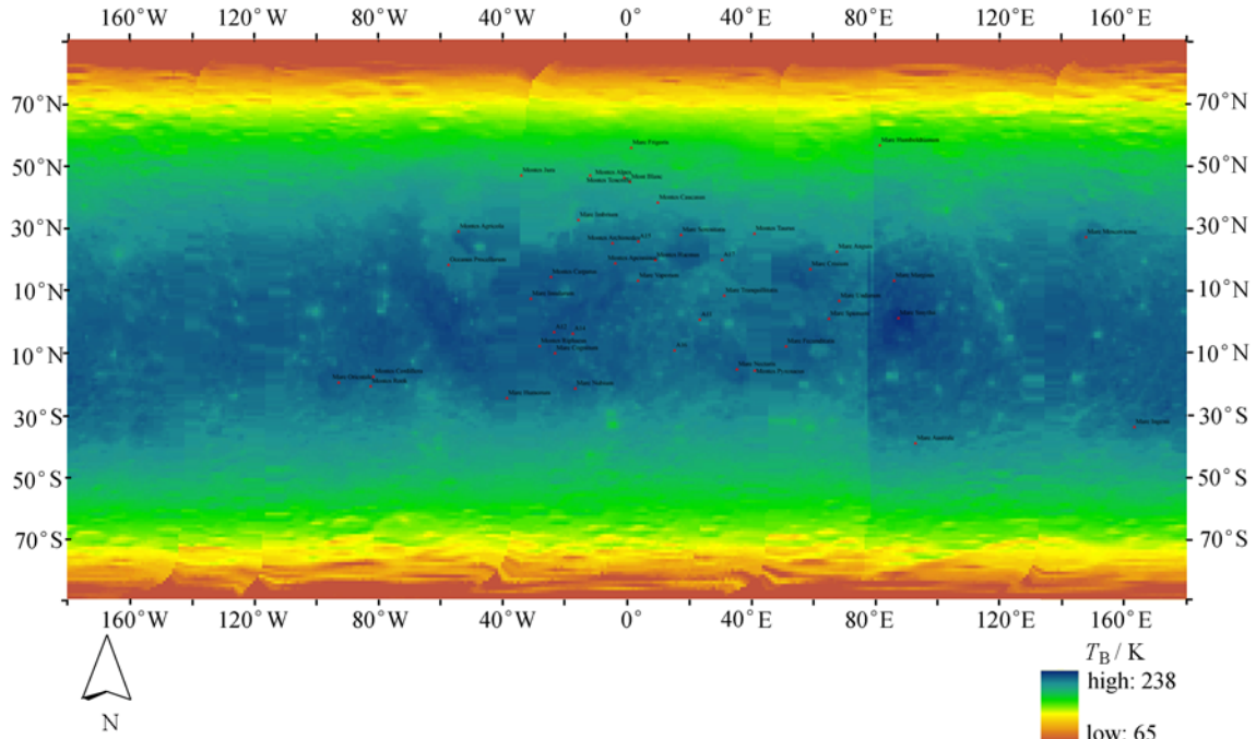
Figure 10 Lunar nighttime brightness temperature of the Moon at frequency of 37.0 GHz.
