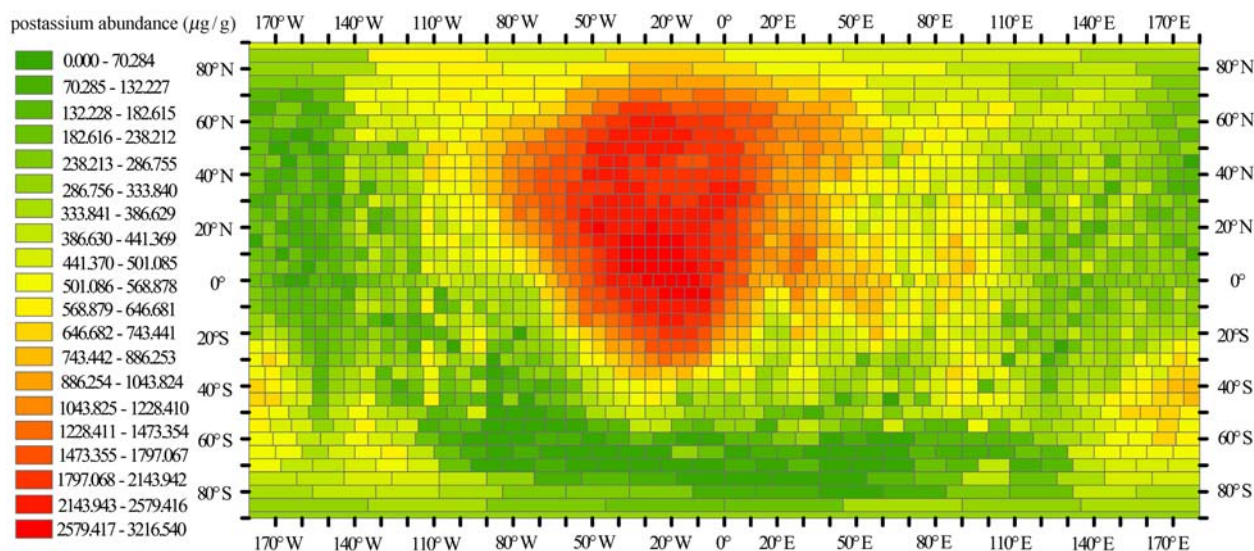
Figure 9 Global map of Potassium abundance (a pixel is 5^\circ \times 5^\circ for longitude and latitude).
