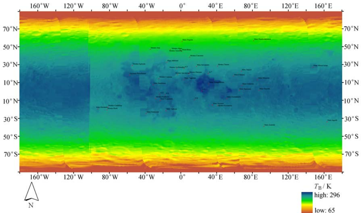
Figure 11 Lunar daytime brightness temperature of the Moon at frequency of 37.0 GHz.
